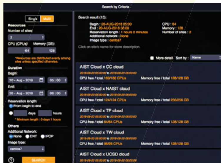
Figure 7: Screenshot of the new multi-site advanced searching functionality in the PRAGMA Cloud Scheduler GUI. Multiple choices are shown for a request of a total of 64 CPUs and 128 GB of memory—the users can select the best one that suits their requirements.
